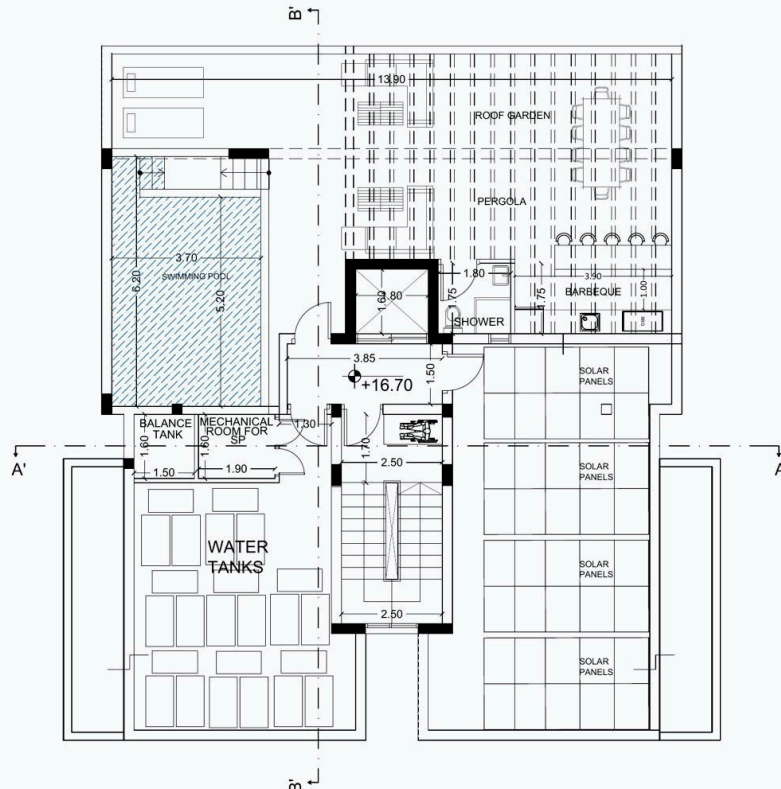
ROOF PLAN
