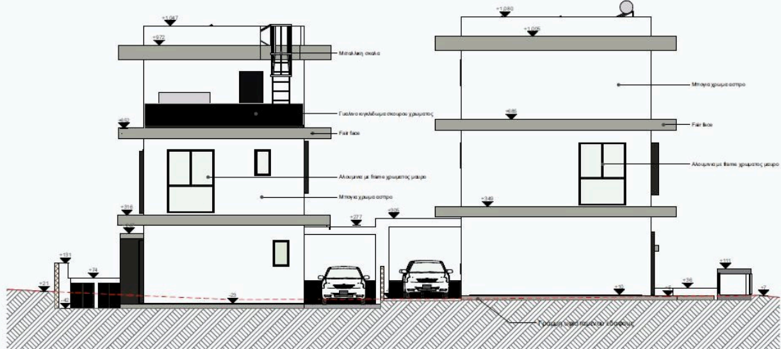
WEST ELEVATION
