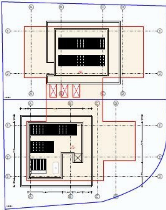
ROOF PLAN / COVERAGE
