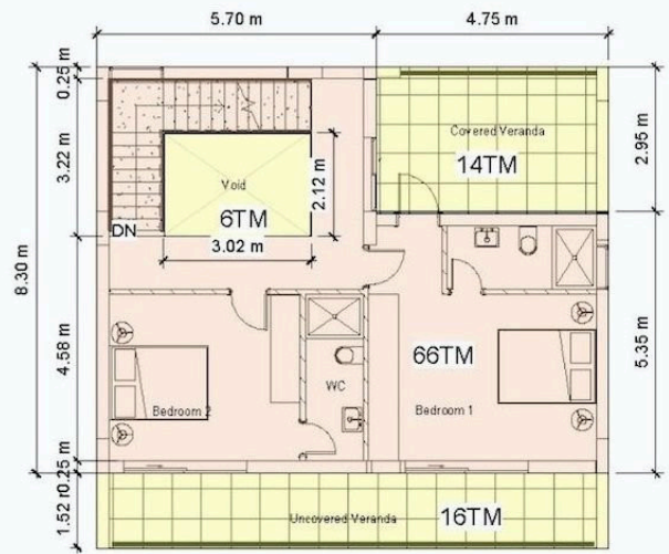
2 H15 1ST FLOOR
