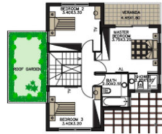
FIRST FLOOR HOUSE TYPE A
