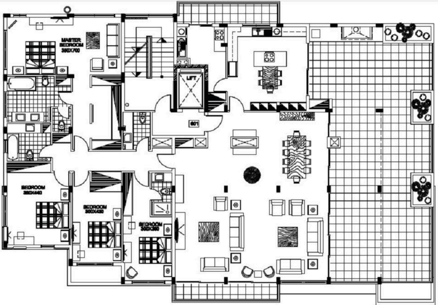
6th floor level
